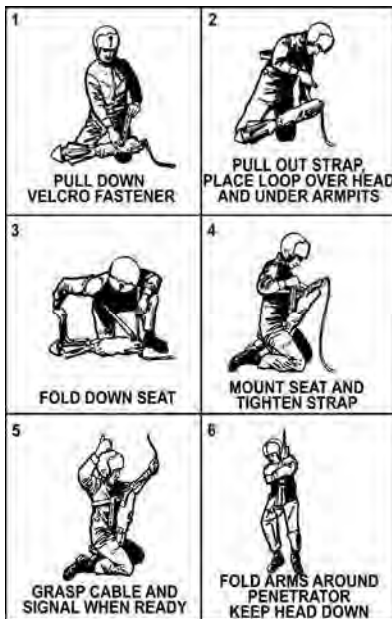
Figure IV-2. Forest Penetrator
