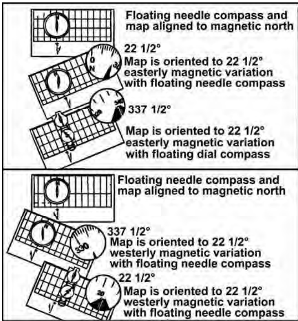
Figure II-4. Map Orientation with a Dial or Needle Compass
