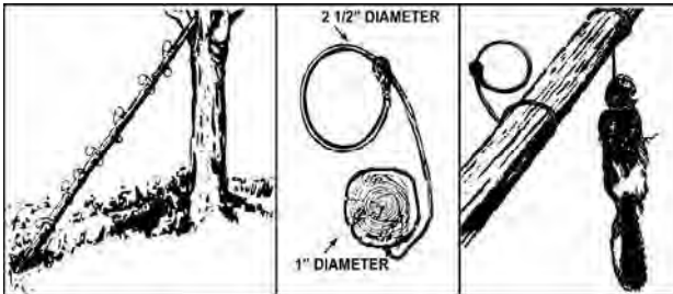
Figure VIII-3. Squirrel Pole
