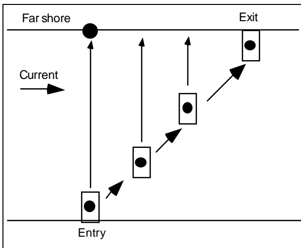
Figure 7-8. Downstream sideslip
