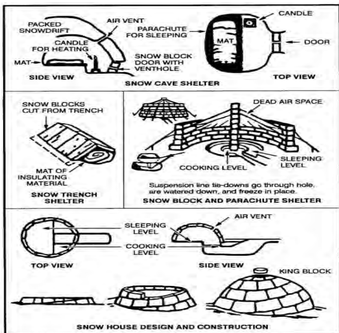
Figure 15-4. Snow houses.
